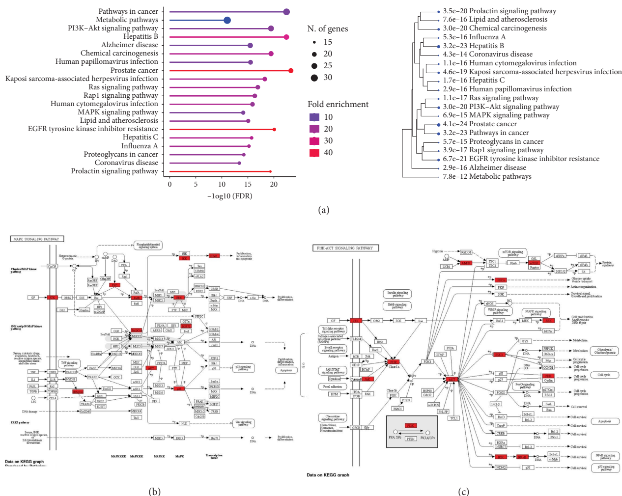
FIGURE 4: (a): Bubble plot of enriched pathways with hierarchical clustering. (b): MAPK signaling pathways. (c): PI3K-AKT signaling pathway.
