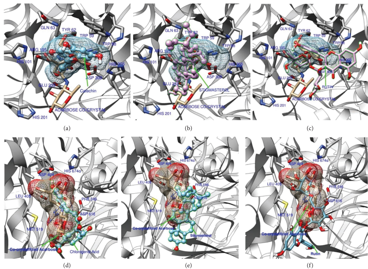
FIGURE 7: Molecular docking study on human pancreatic α-amylase (1B2Y) with (a) catechin, (b) stigmasterol, (c) rutin and human lysosomal α-glucosidase (5NN8) with (d) chlorogenic acid, (e) stigmasterol, and (f) rutin.
